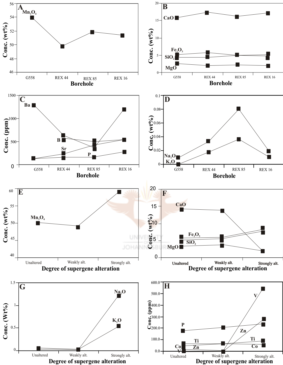
Figure 4.5. A-D: Lateral geochemical trends in C-zone unaltered braunite lutite observed from south (G558) to north (Rex 16) in the study area. E-H: Geochemical trends observed for the M-Zone with increasing degree of supergene alteration. Reference boreholes selected are Rex 85 (unaltered braunite lutite), Rex 70 (weakly supergene altered braunite lutite) and Rex 2 (strongly supergene altered braunite lutite).
