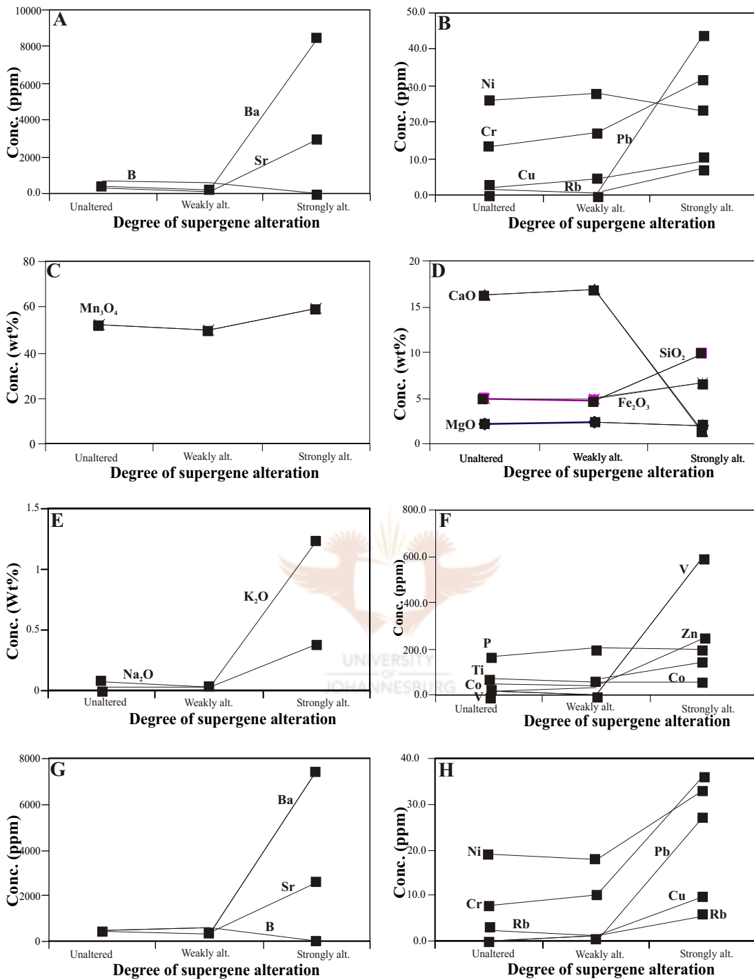
Figure 4.6. A-B: Lateral geochemical trends observed in M-zone with increasing degree of supergene alteration (continue from Fig. 4.5). C-H: Geochemical trends observed for C-Zone with increasing degree of supergene alteration. Reference boreholes selected are Rex 85 (unaltered braunite lutite), Rex 70 (weakly supergene altered braunite lutite), and Rex 2 (strongly supergene altered braunite lutite).
