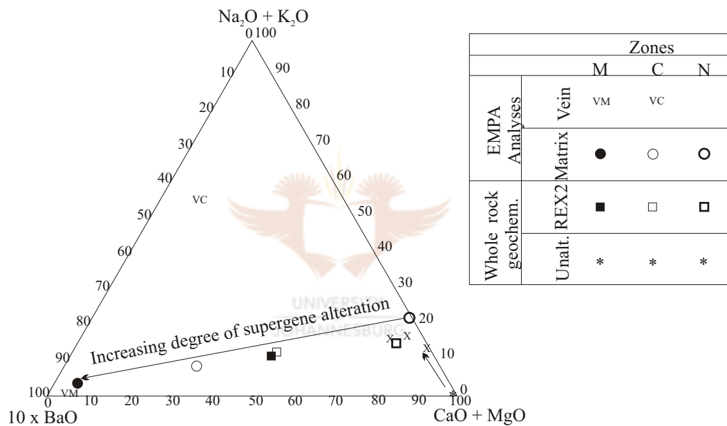
Figure 5.3. Ternary plot of \text{Na}_2\text{O} + \text{K}_2\text{O} , \text{CaO} + \text{MgO} and \text{BaO} contents of the matrix, cross-cutting veinlets and whole rock composition of Rex 2 and an unaltered sample (Unalt.) of the lithostratigraphic M, C and N-Zones. The composition of todorokite in Rex 2 is compared to the composition of todorokite reported by Gutzmer and Beukes (2000) (indicated by x).
