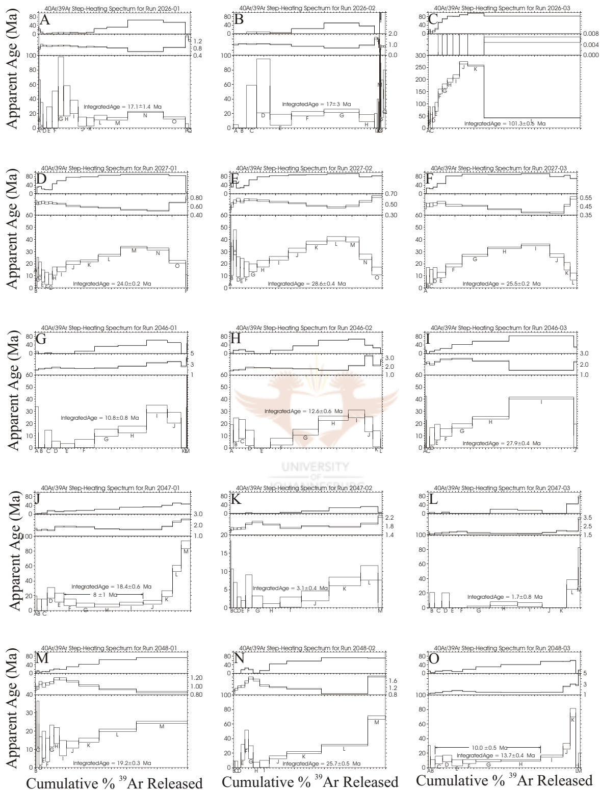
Figure 5.4 (A-F): Step heating spectra for three distinct todorokite and manganomelane grains of two representative samples from the M-zone. (G-O): Step heating spectra for three distinct todorokite and manganomelane grains of three representative samples from the C-zone.
