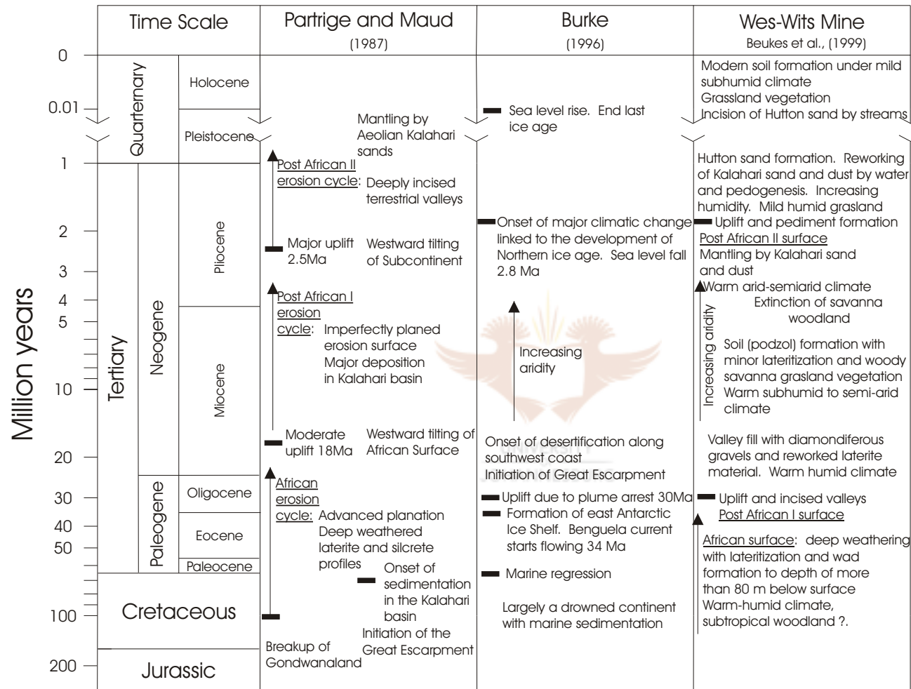
Figure 6.3. Recent concepts for Post-Gondwana landscape evolution in Southern Africa by Beukes et al. (1999), Burke (1996), and Partridge and Maud (1987) (diagram modified after Beukes et al., 1999)
