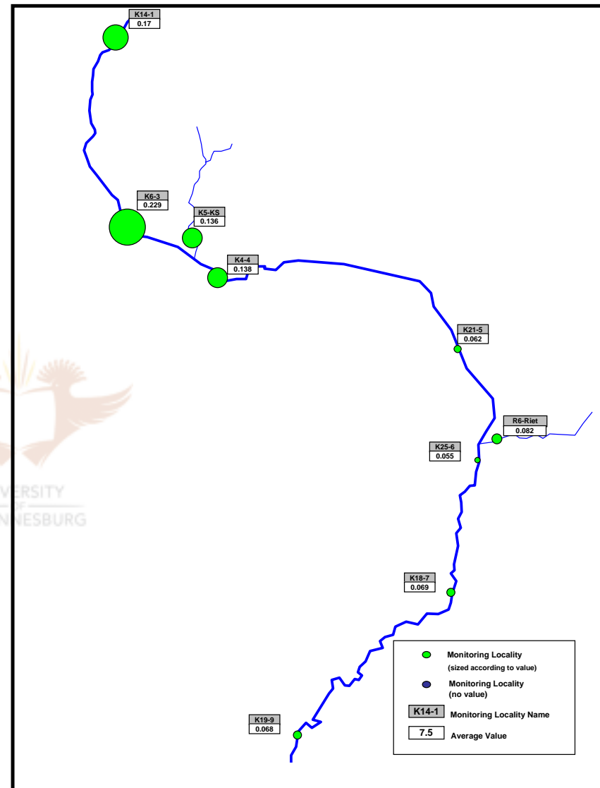
Appendix 3.41: Spatial trends in average nickel (mg/l) in the Klip River catchment (1973 to 2001).
