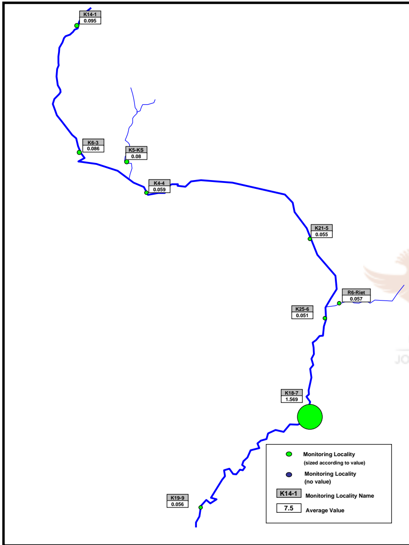
Appendix 3.40: Spatial trends in average cobalt (mg/l) in the Klip River catchment (1973 to 2001).
